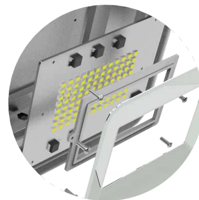
PCB (LED + Integrated Driver)
